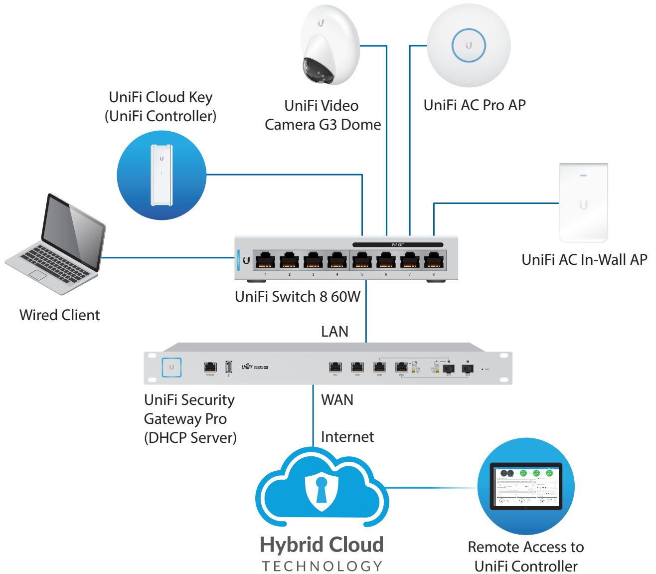
US-8-60W Sample Network Diagram
