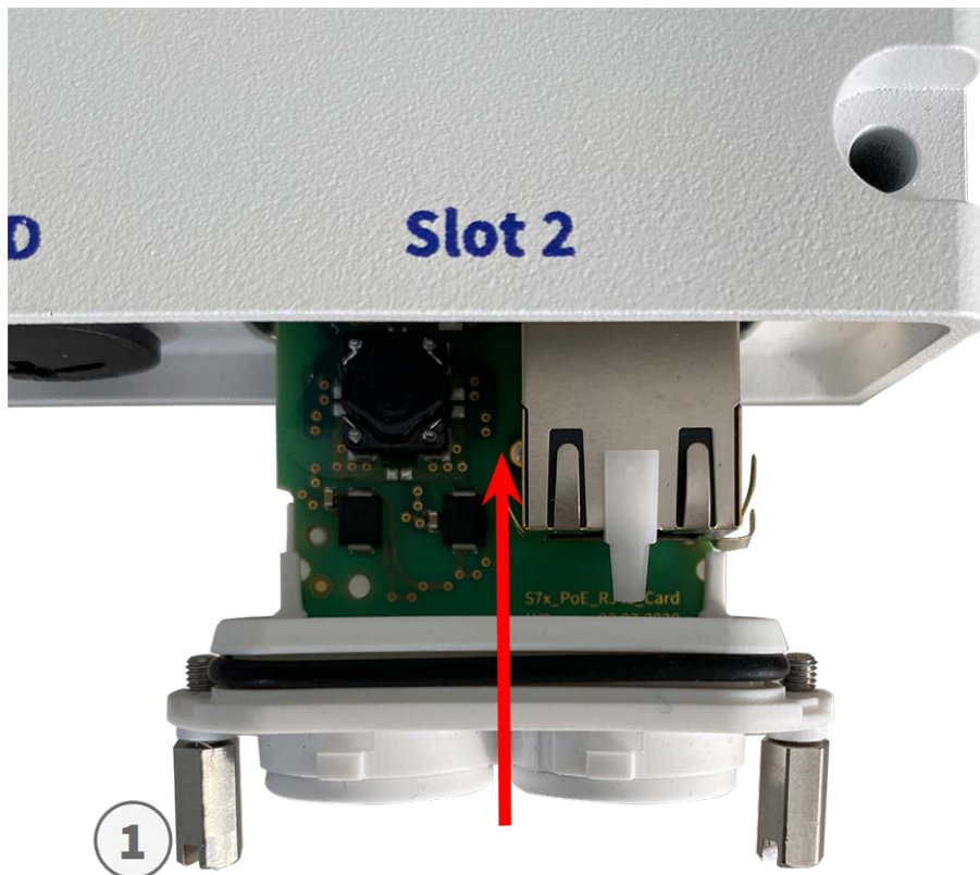
Fig. 19: Connecting the Interface Board RJ45
