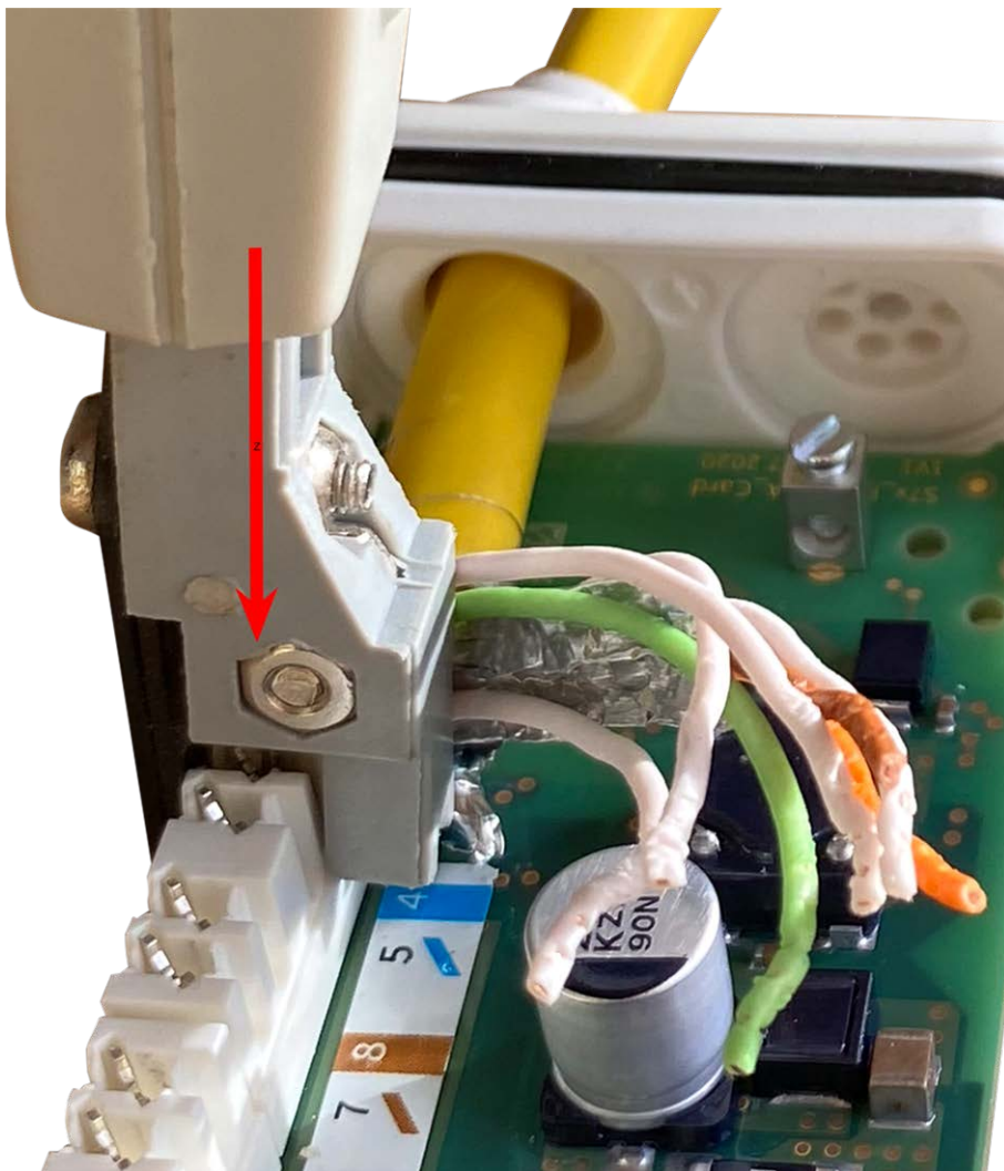
Fig. 26: Network wires connected using LSA+/Krone tool
