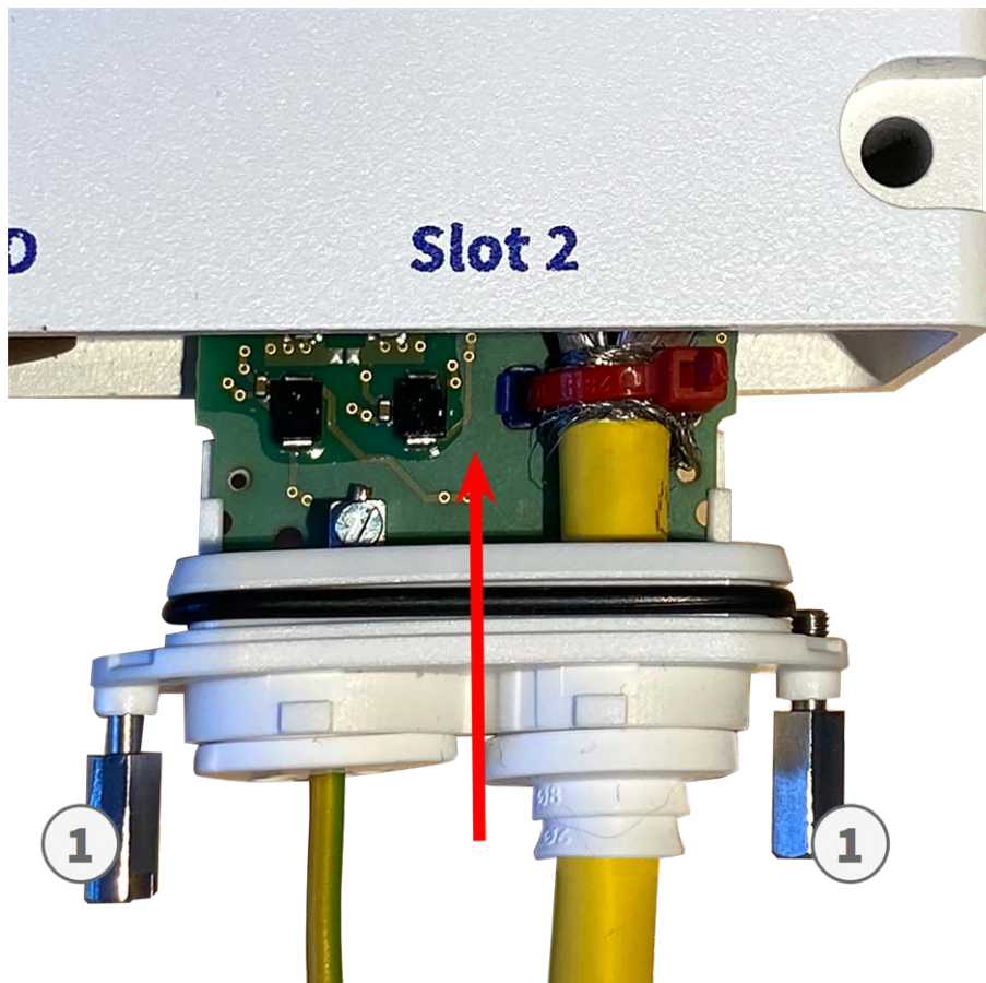
Fig. 30: Connecting the Interface Board LSA
