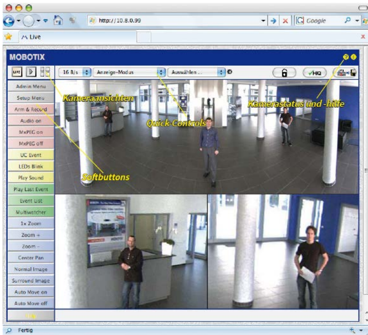
Fig. 49: The interface of the camera software
