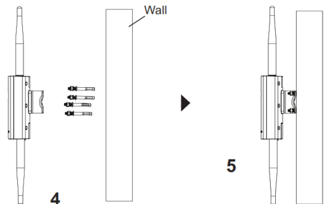
Figure 19: GWN7630LR Wall Mount
