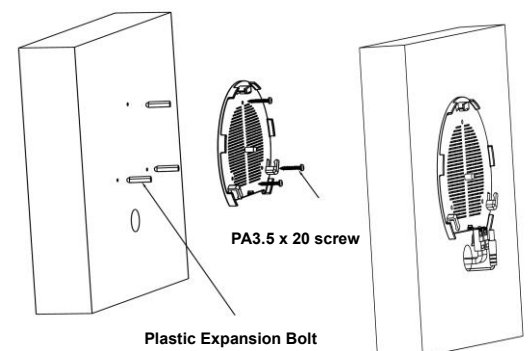
Figure 9: Wall Mount – Steps 1 & 2
