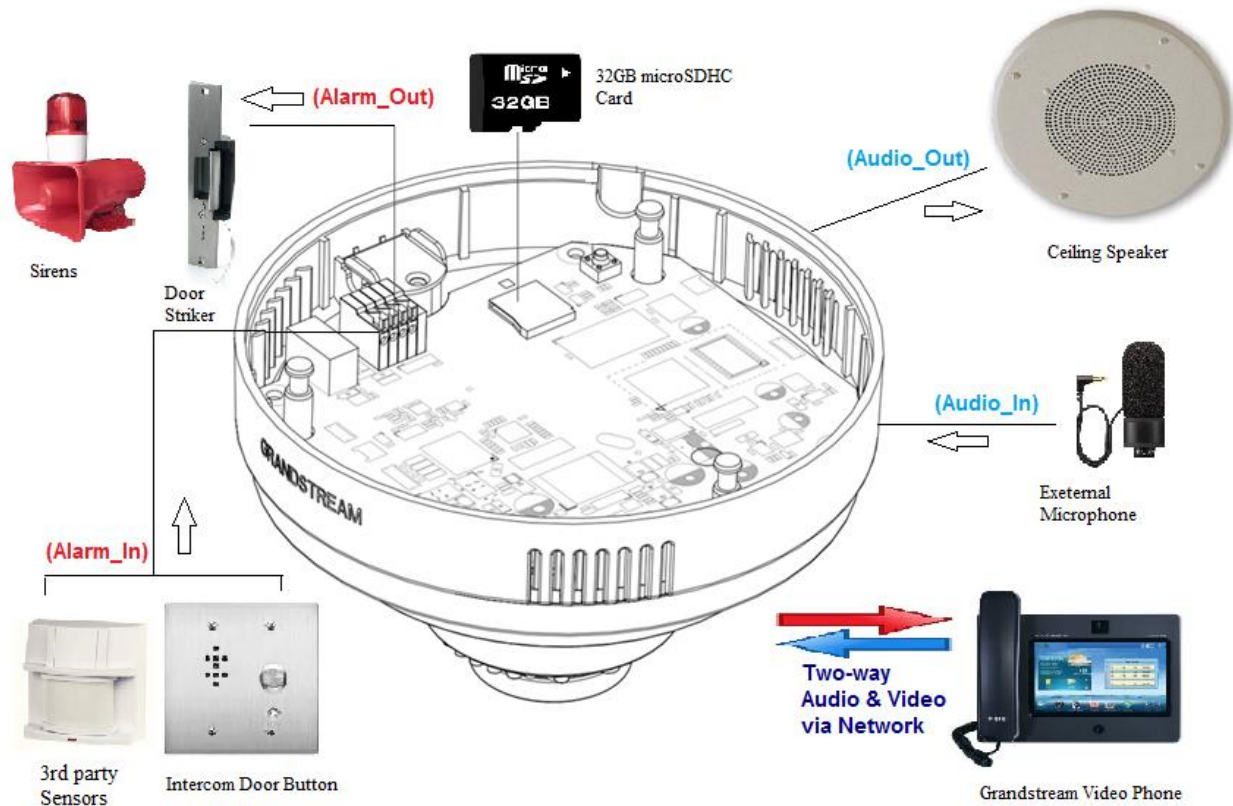
Figure 7-1: Application Peripheral Connection for GXV3611IR_HD
