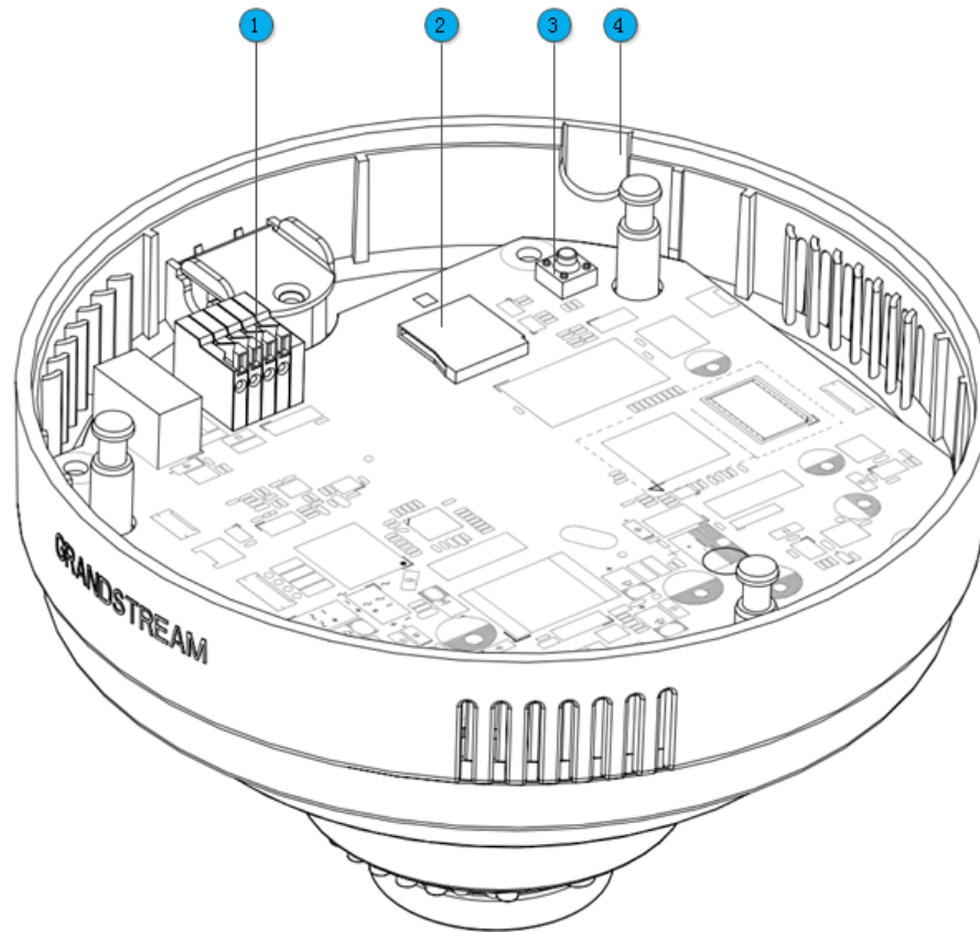
Figure 2: GXV3611IR_HD Inside View
