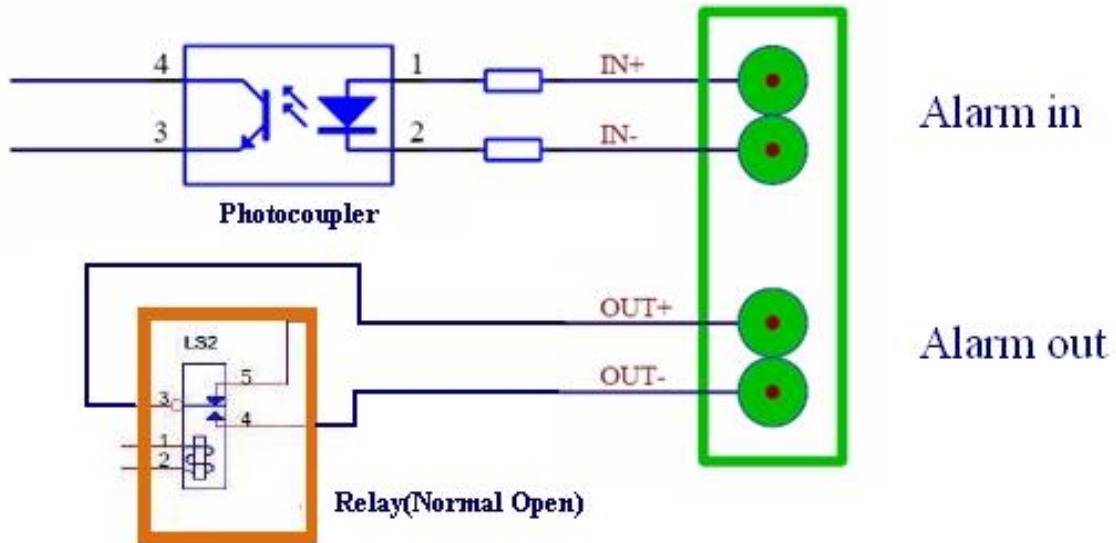
Figure 7-2: Alarm_In and Alarm_Out Connection Circuit Sample for GXV3611IR_HD
