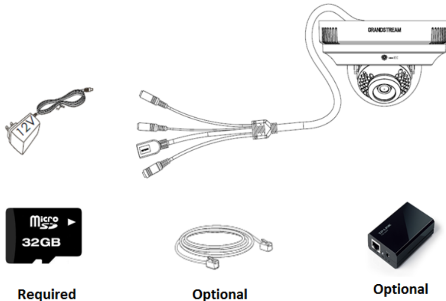
Figure 6-1: GXV3611IR_HD Standalone Application
