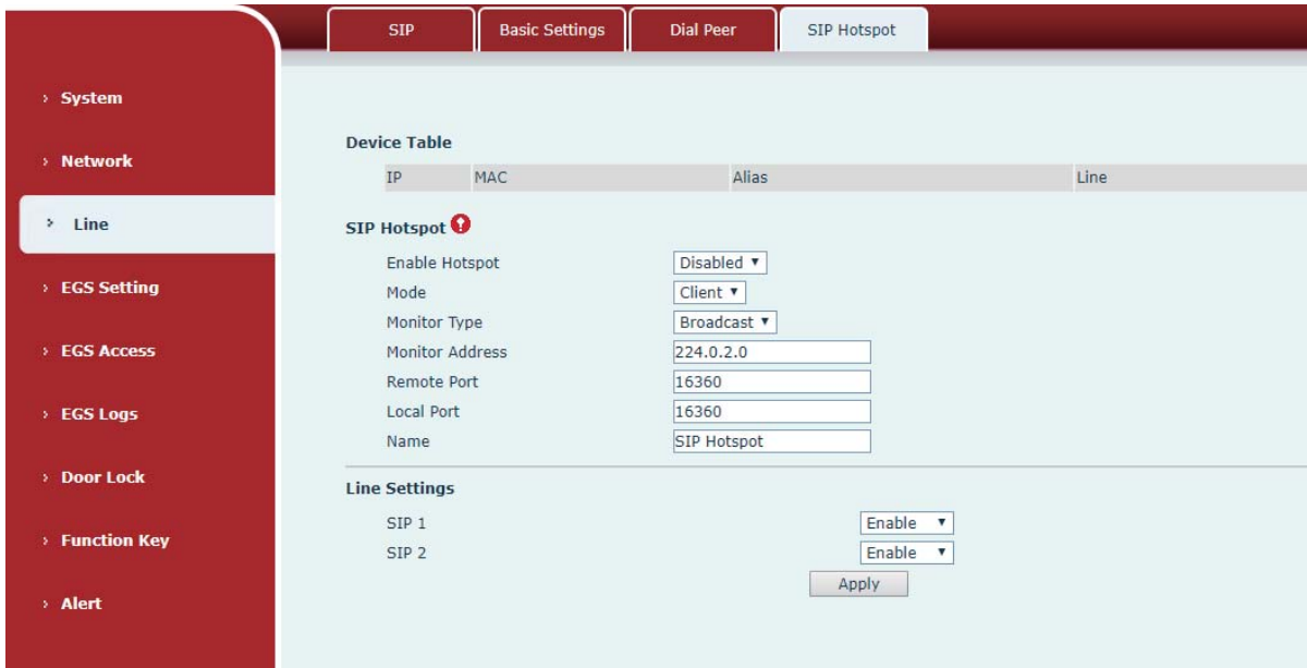
Figure 13 - SIP Hotspot
