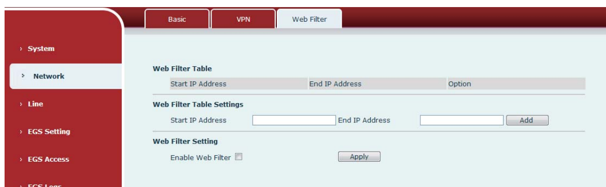
Figure 22 - WEB Filter
