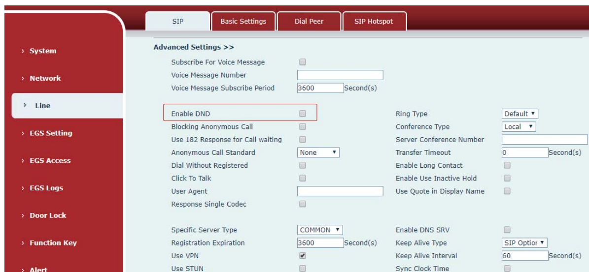
Figure 9 - Enable DND
