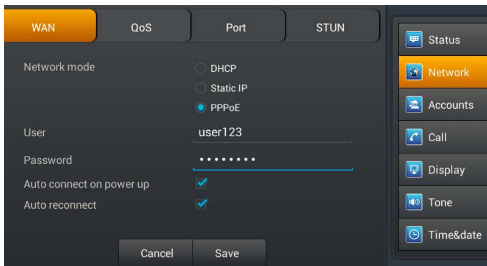
PPPoE interface
