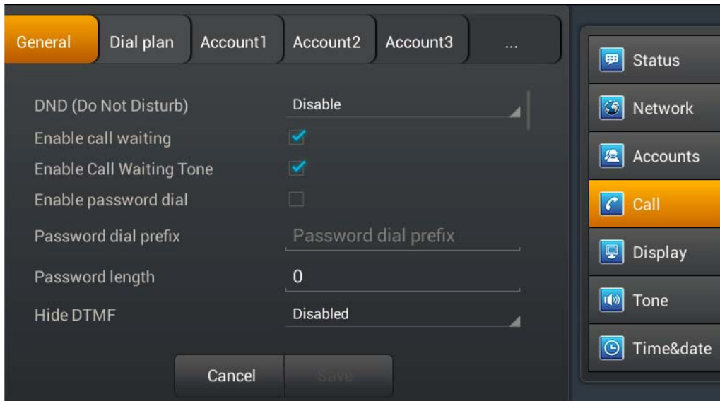
General interface
