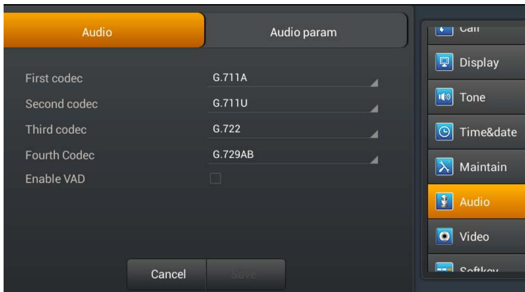
Audio interface
