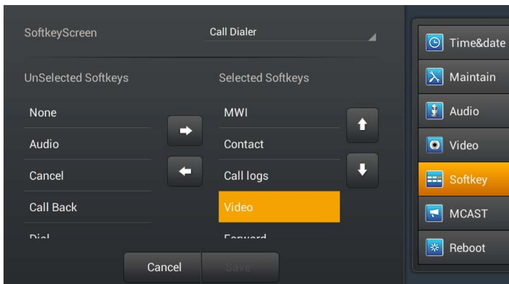
Softkey interface
