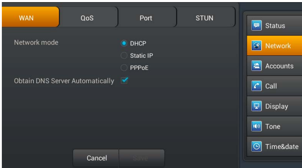
DHCP interface
