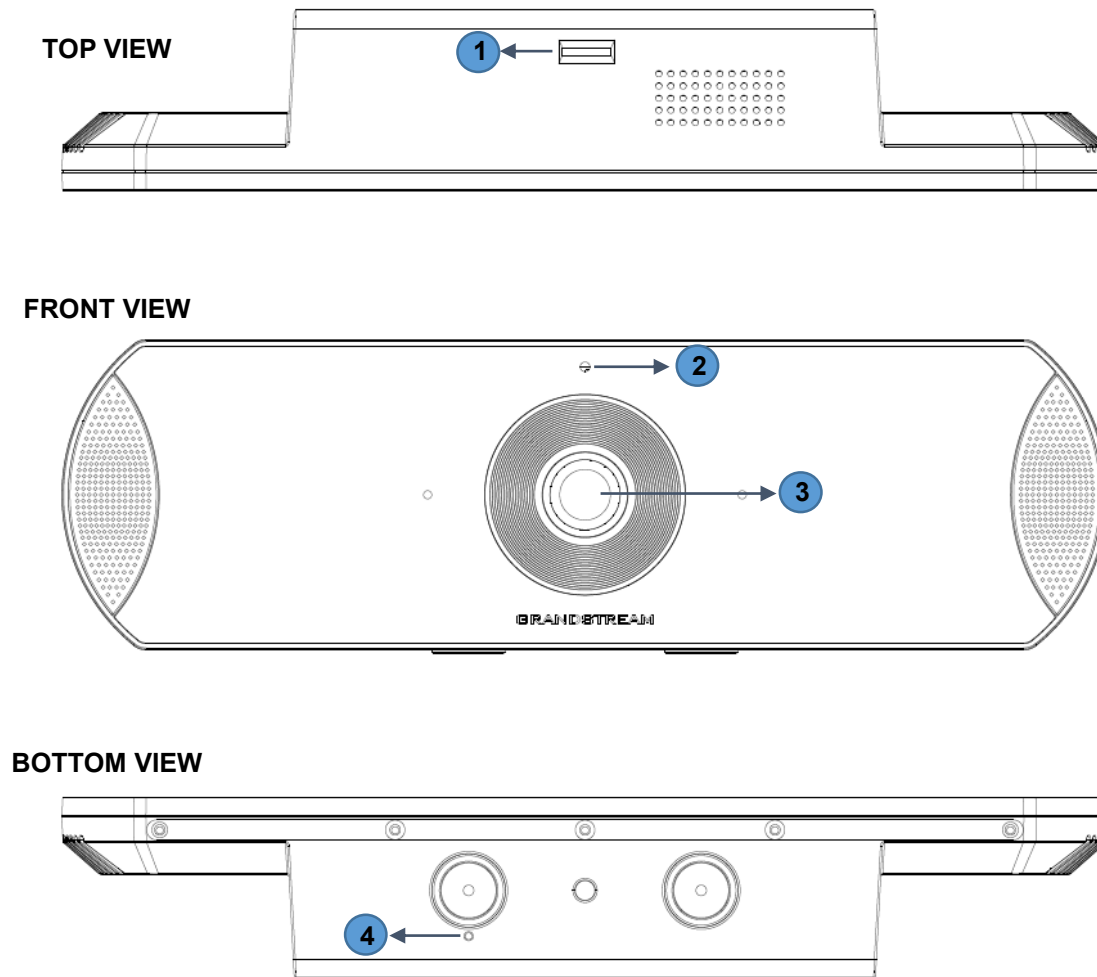
Figure 2:GVC3210 Front/Top/Bottom Panel
