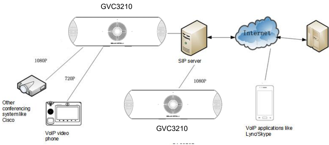
Figure 5: Deploy GVC3210 with other Devices
