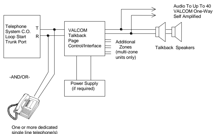
Block Diagram for Loop Start Trunk Port And/Or Single Line Telephone Access of a Valcom Talkback Page Control/Interface
